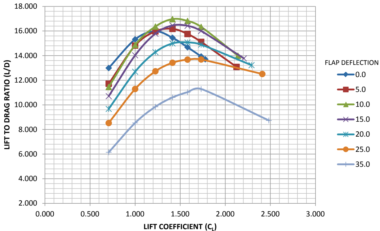
Figure 5.24 – 765-095-TS3 - Low Speed Lift / Drag; Free Air
