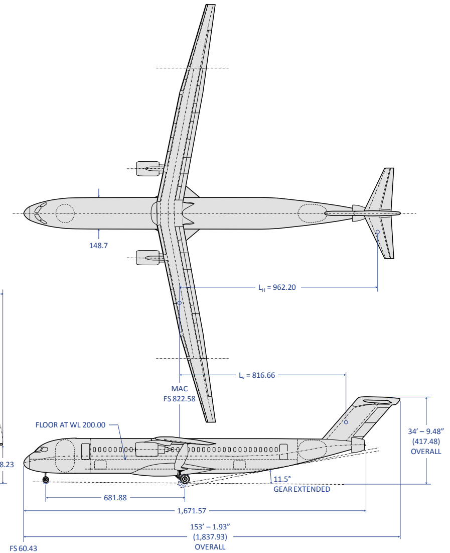
Figure 5.26 – 765-095-TS4 - Truss Braced Wing with LNG Fuel Cell BLI
