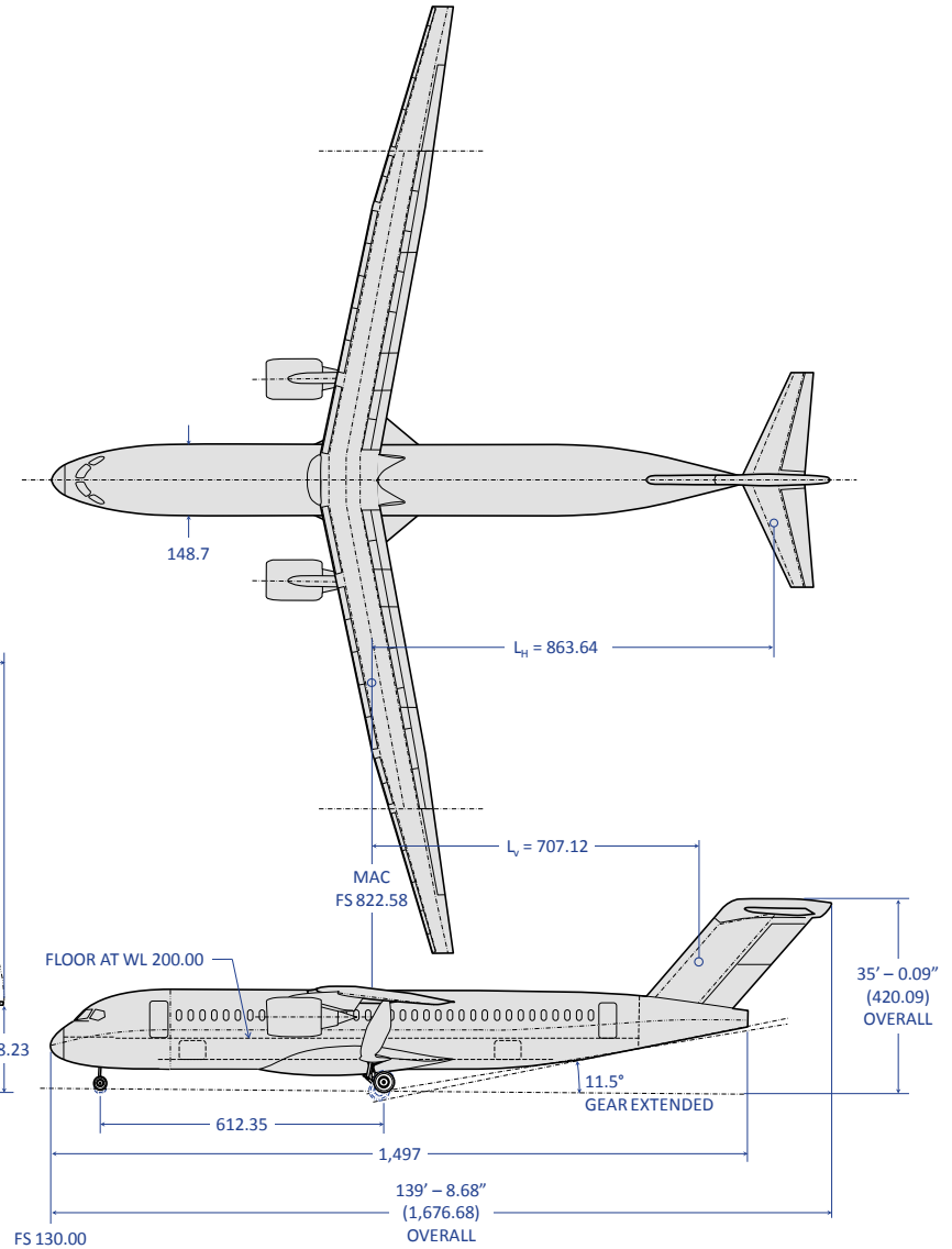
Figure 5.6 – 765-095-TS1 – Truss Braced Wing with gFan++
